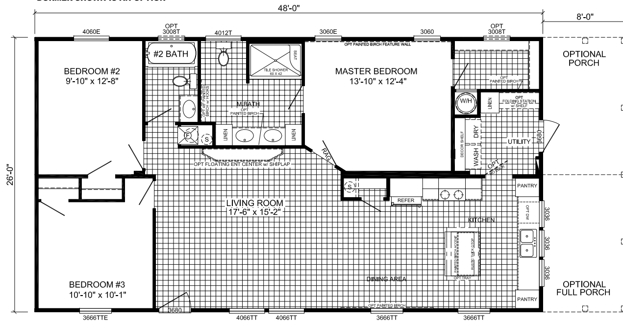
H-2483N-XT 3-BEDROOM / 2-BATH 28 x 52 - Approx. 1248 Sq. Ft.
